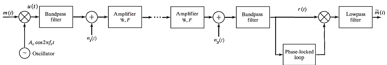
Figure 1: DSB modulation in a channel with cascade of amplifiers.
